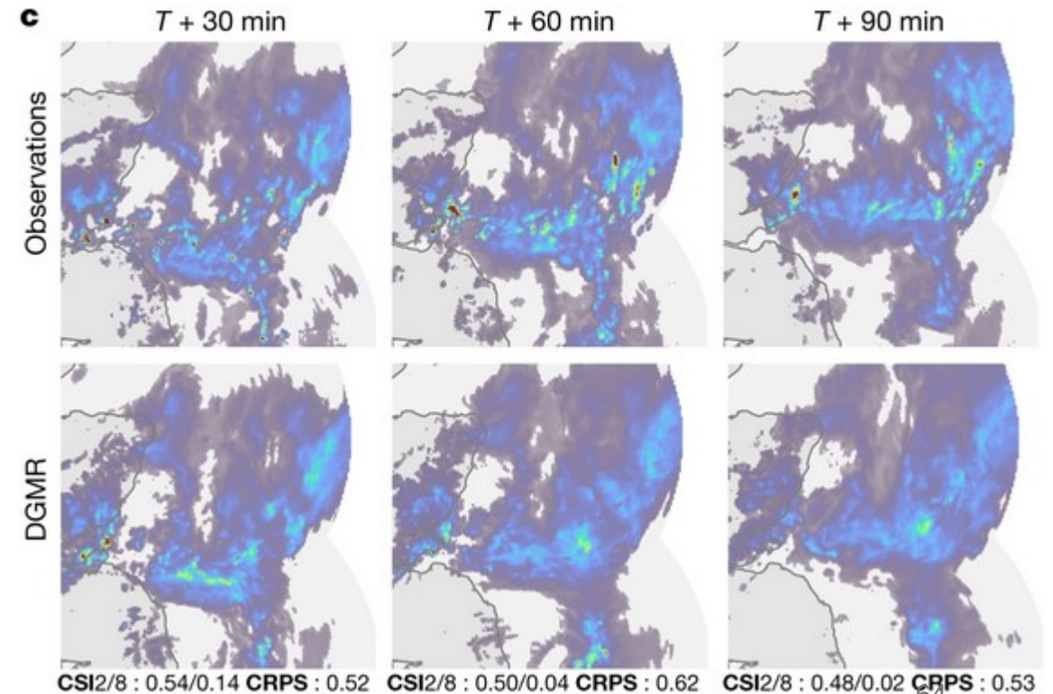
Obs (top) and AI prediction (bottom) for UK rain
