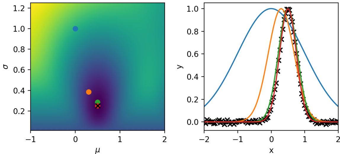
Newton-Raphson
